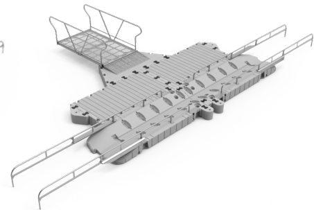
EZ Launch® Drive Thru with Small Platform
